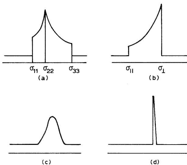
Fig. 2. NMR lineshape of polycrystalline solid samples. (a) Anisotropic, three chemical shift values; (b) axially symmetric, two chemical shift values; (c) insufficient averaging by slow sample rotation; (d) sharp signal by sufficient averaging by rapid rotation.
